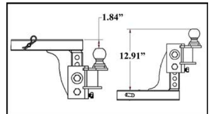
Figure 2: Hitch bar can be used in the raised or dropped position.
