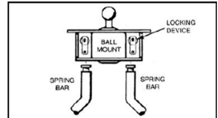
Figure 5: WD spring bars attached to head through socket and secures with clip.
