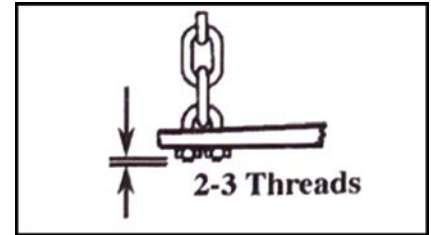
Figure 4: Let 2-3 threads of u-bolt through the bottom of each lock nut.
