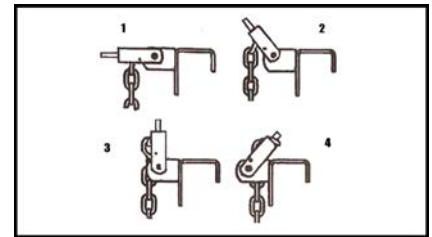
Figure 14: Raise the lift bracket with the chain and secure with locking pin.
