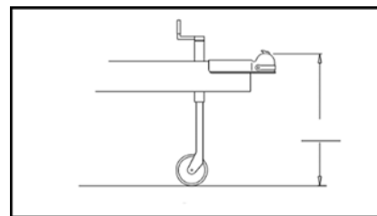
Figure 8: On a level surface, measure the height of your trailer coupler to ground.
