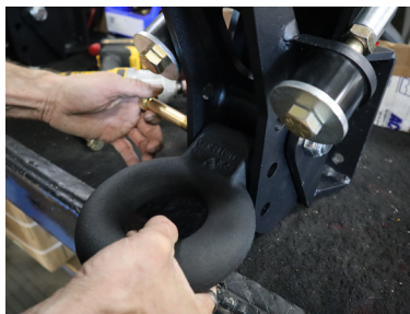
Figure 1: Line Up Pintle Ring with Shocker Hitch
